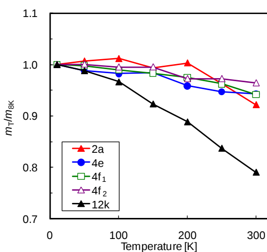
Fig.2 Thermal variation of the magnetic moments ( m_T ) of iron ions on five sublattices in \text{Sr}_{1-x}\text{La}_x\text{Fe}_{12-x}\text{Co}_x\text{O}_{19} ( x=0 ) relative to the magnetic moments at 8K ( m_{8K} ).
