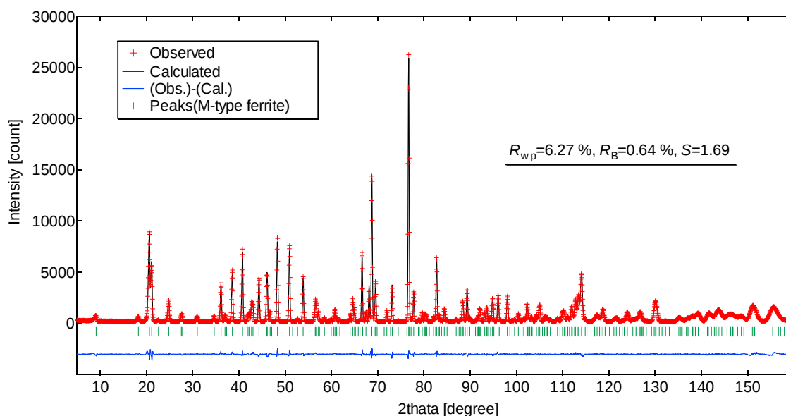
Fig.1 Typical result of Rietveld analysis of powder neutron diffraction pattern of \text{Sr}_{1-x}\text{La}_x\text{Fe}_{12-x}\text{Co}_x\text{O}_{19} ( x=0 ) obtained at 8 K.
